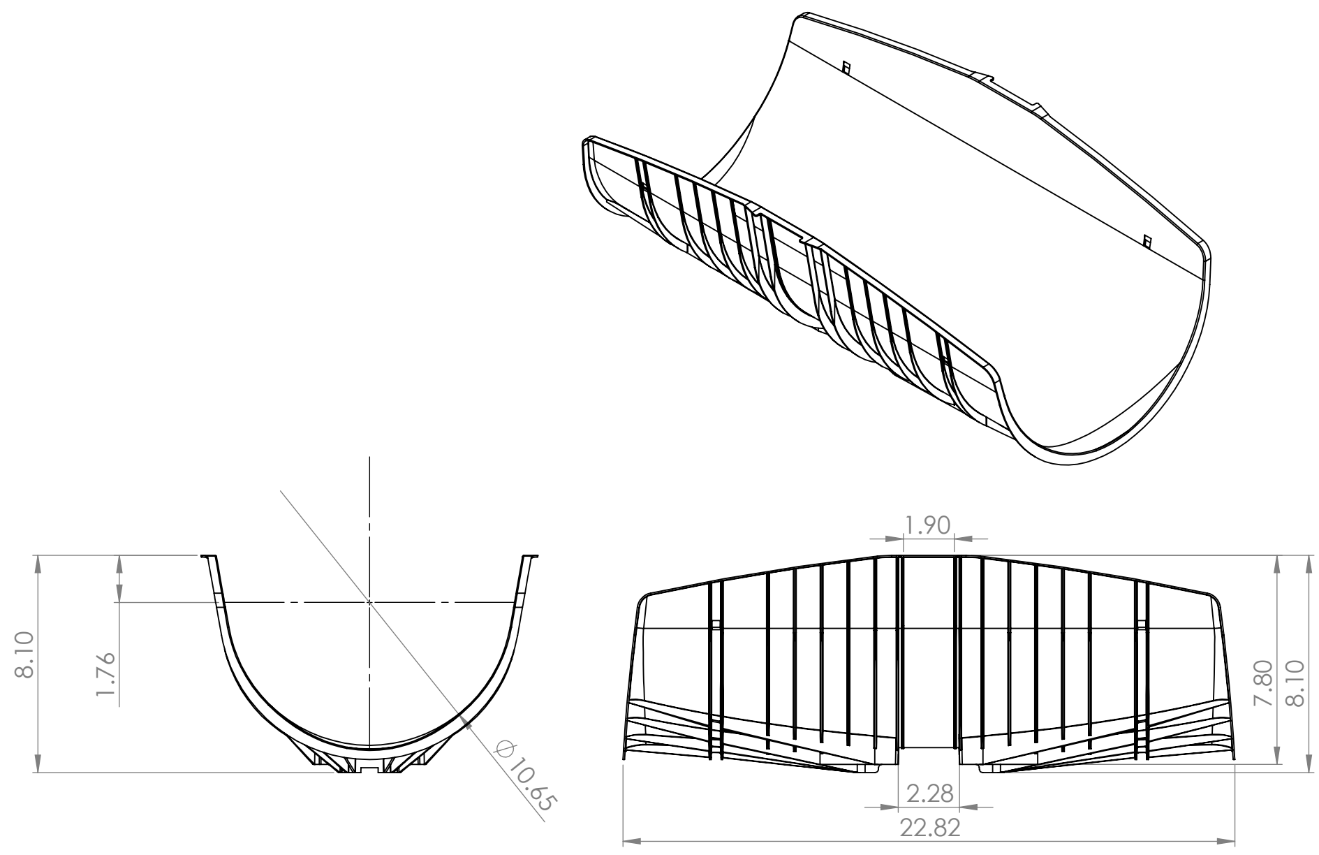
INSUGUARD MULTI IMI050G NOT TO SCALE
