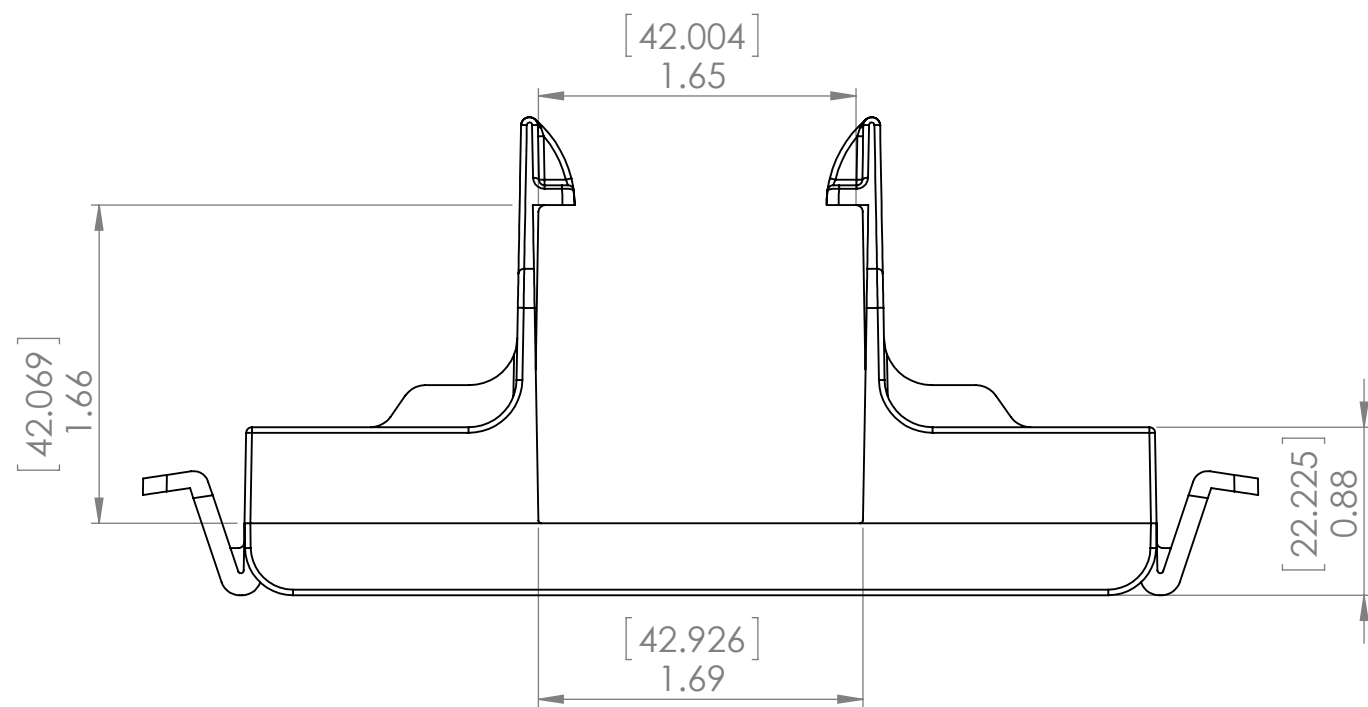
STRUT 42x42 - IM42X42 NOT TO SCALE
