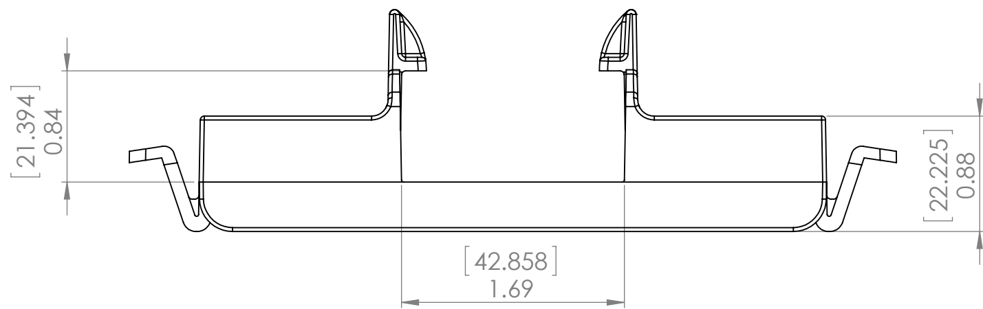
STRUT 42x20 - IM42X20 NOT TO SCALE
