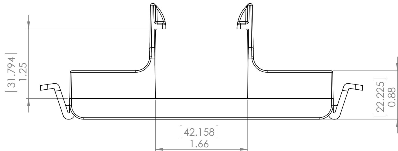
STRUT 31x43 - IM31X43 NOT TO SCALE
