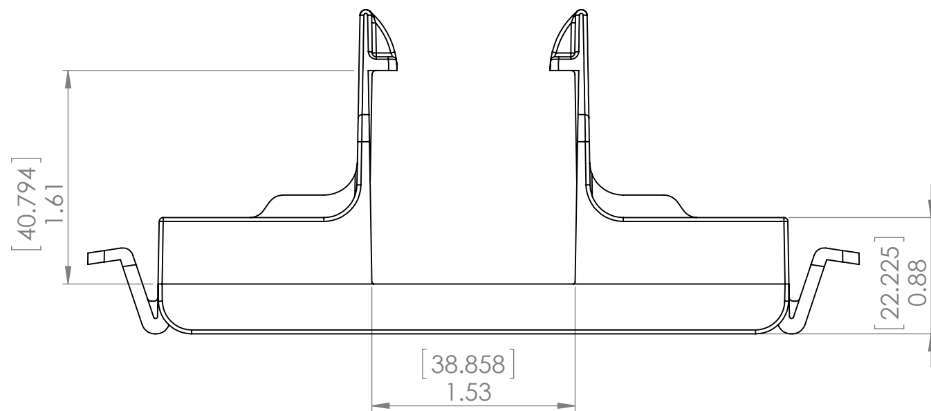
STRUT 40X38 - IM40X38 NOT TO SCALE
