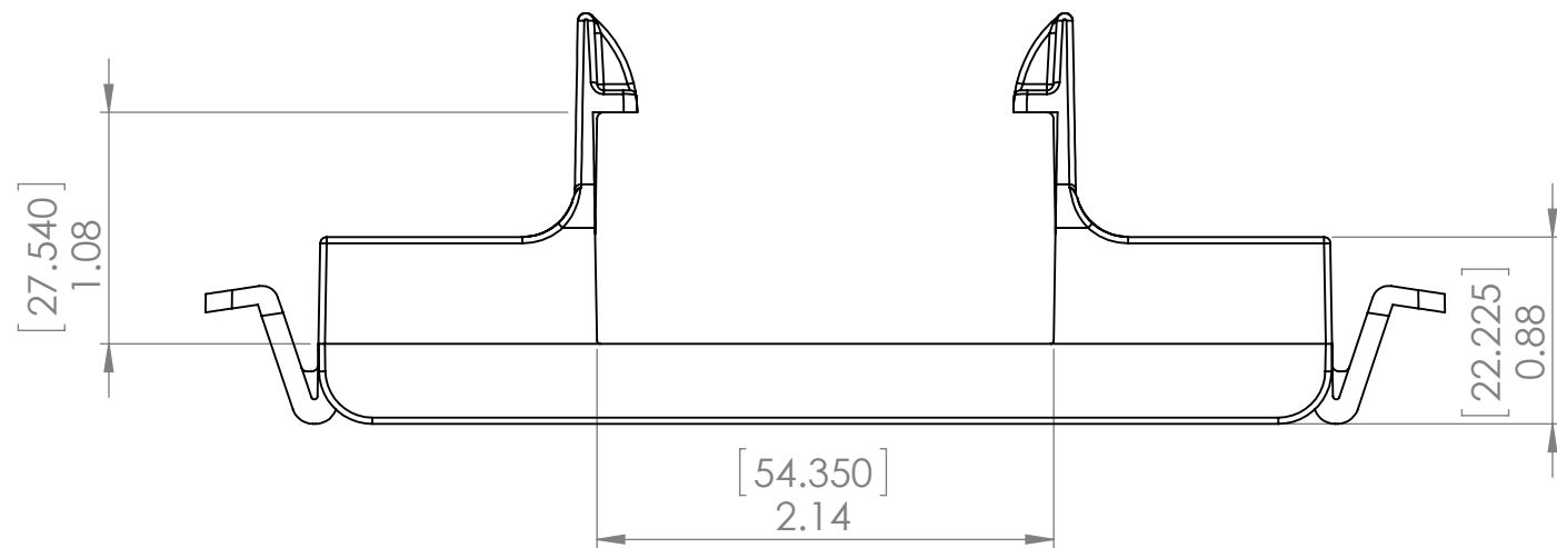
STRUT 54X27 - IM4D2I NOT TO SCALE
