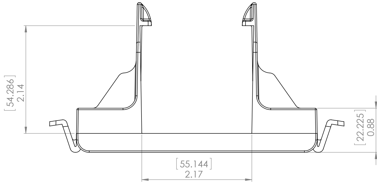
STRUT 54X54 - IM4D22 NOT TO SCALE
