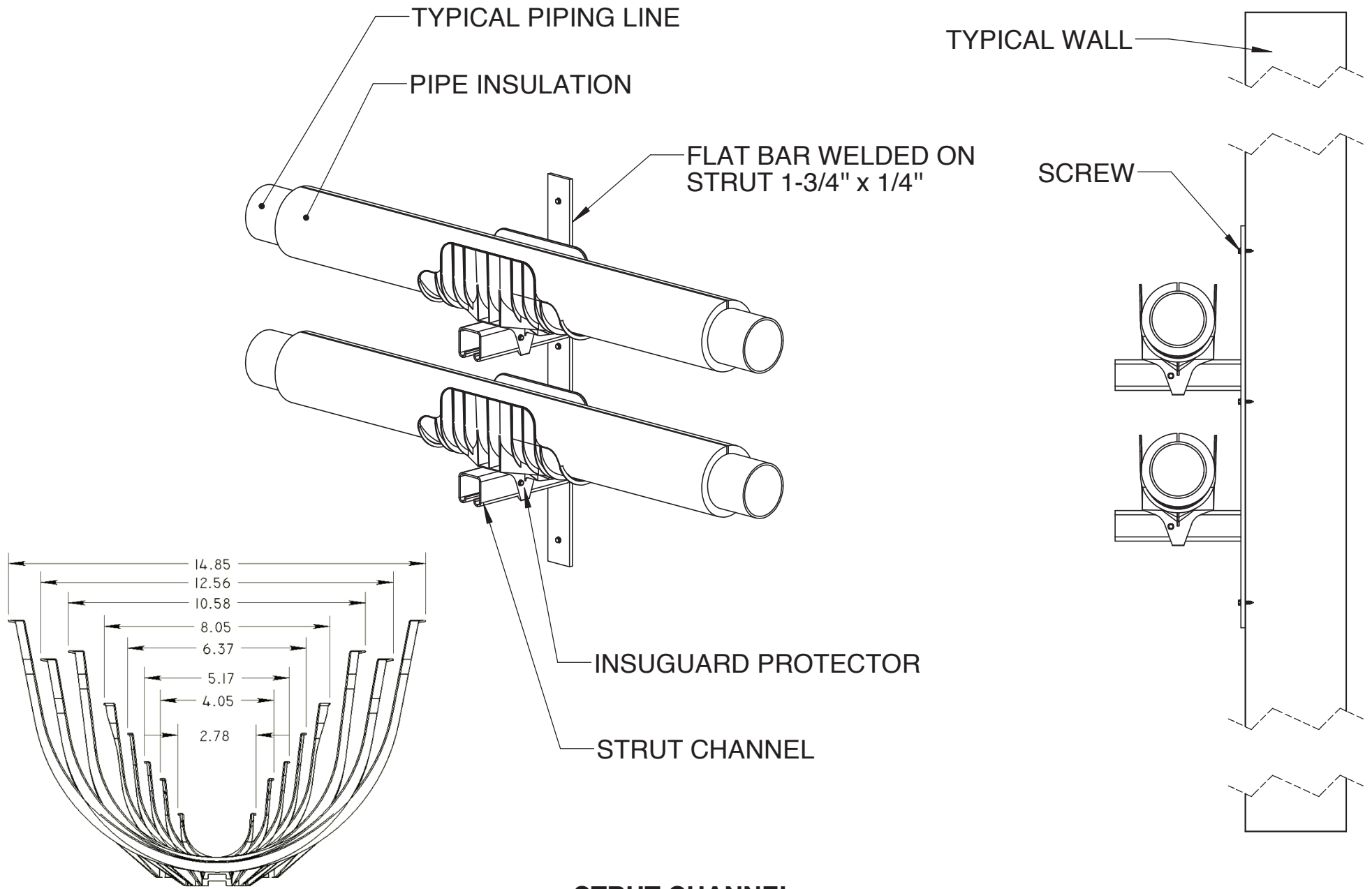
TYPICAL WALL MOUNTING INSTALLATION DETAIL OF PIPING PROTECTOR
