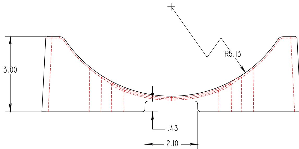
STAB 1050 STRUT STABILIZER NOT TO SCALE
