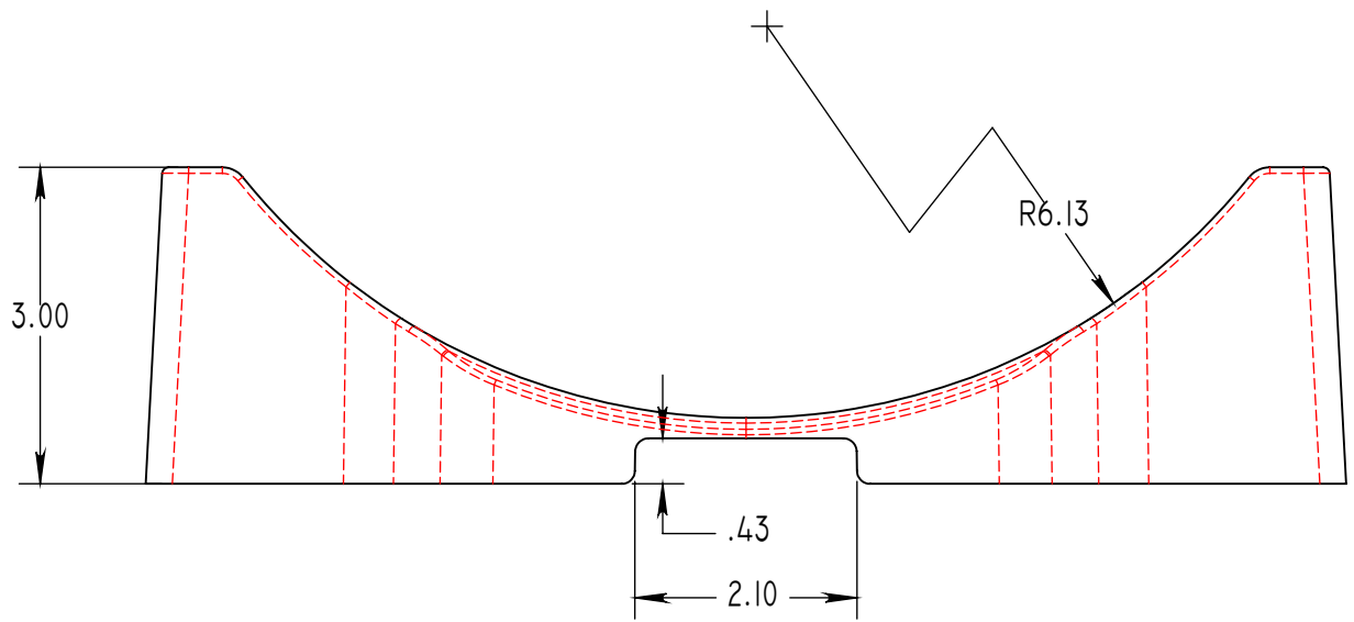
STAB 1250 STRUT STABILIZER NOT TO SCALE
